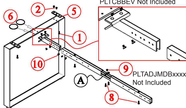
ADJUSTABLE BEAM
