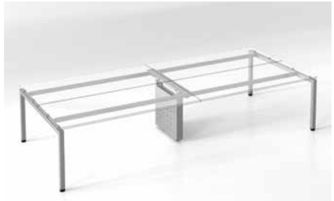
Standard 60" x 144" 4-Person Benching Workstation: PLT3072(4), PLTEGU60(2), PLTEGU4860ILCMB, PLTDB72(4), PLTCBB(2)
